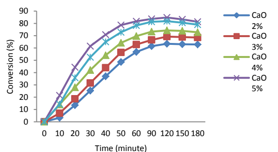
Figure 4a. Effect of catalyst amount on conversion of methyl ester (molar ratio of methanol to oil = 12:1, reaction temperature = 60°C).
