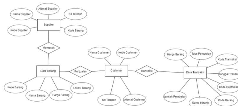
Gambar 1. Entity Relationship Diagram
