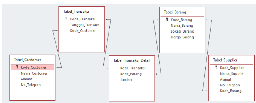
Gambar 5. Contoh Tampilan Relationship
