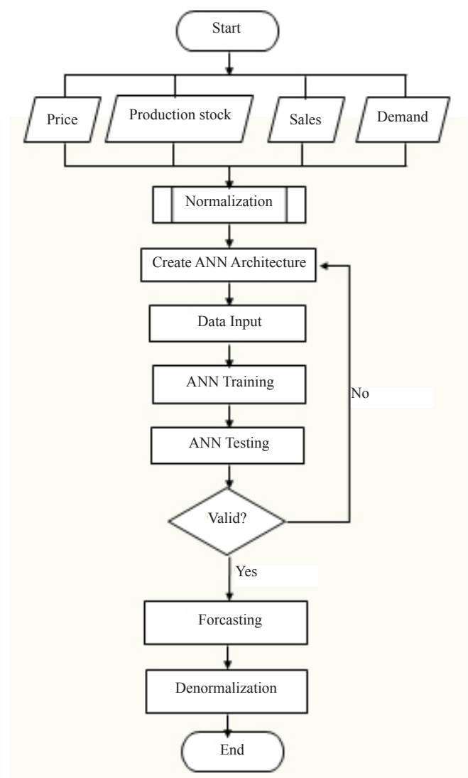
Figure 2. Research framework
