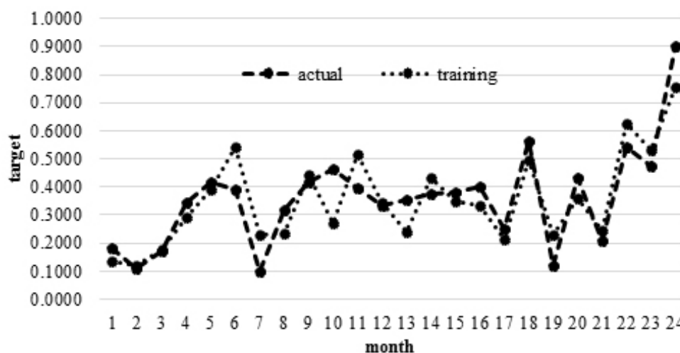
Figure 3. plot of actual demand and training results
